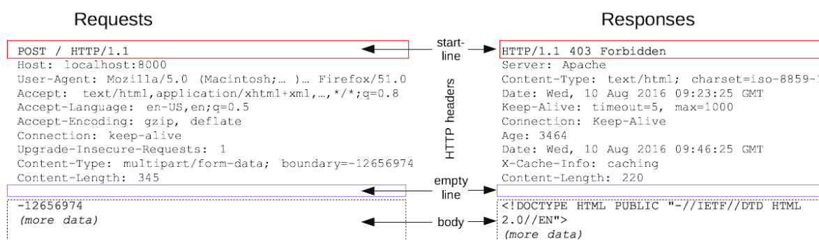
Figura 5: Request - Response
